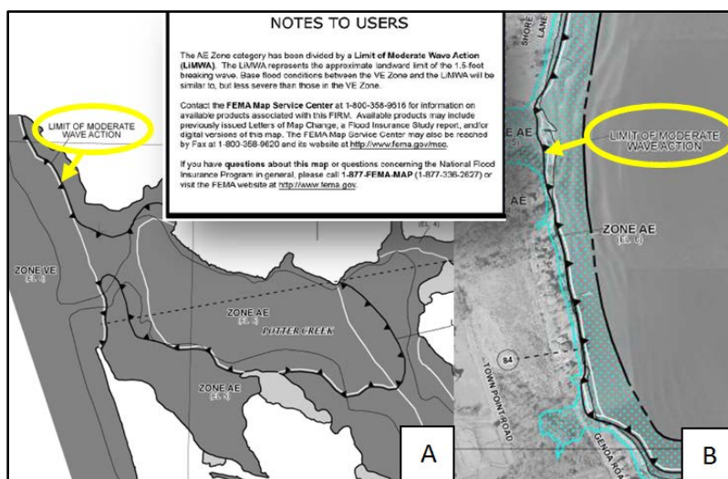
Figure 1: FIRM showing area seaward of the LiMWA
